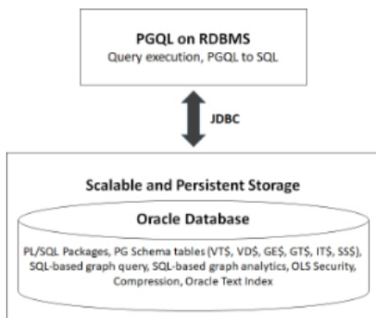
Figure 4-2 PGQL on Oracle Database (RDBMS)
