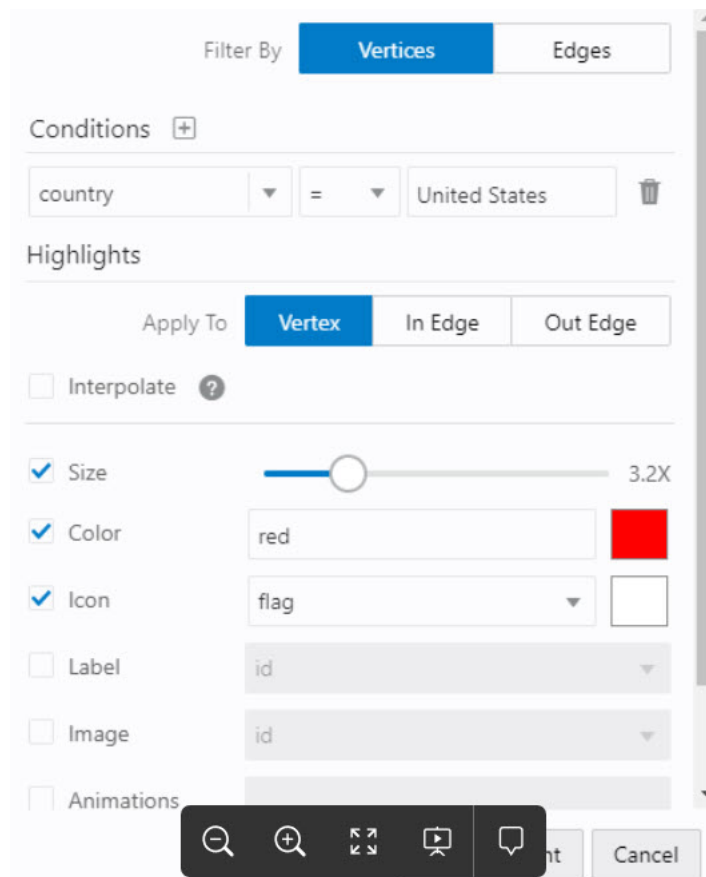
Figure 5-3 Highlights Options for Vertices
