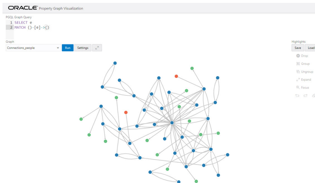
Figure 5-1 Query Visualization
