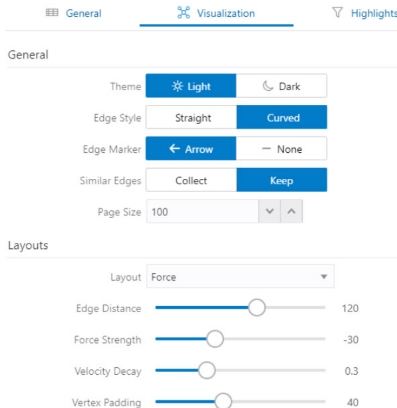
Figure 5-2 GraphViz Settings Window
